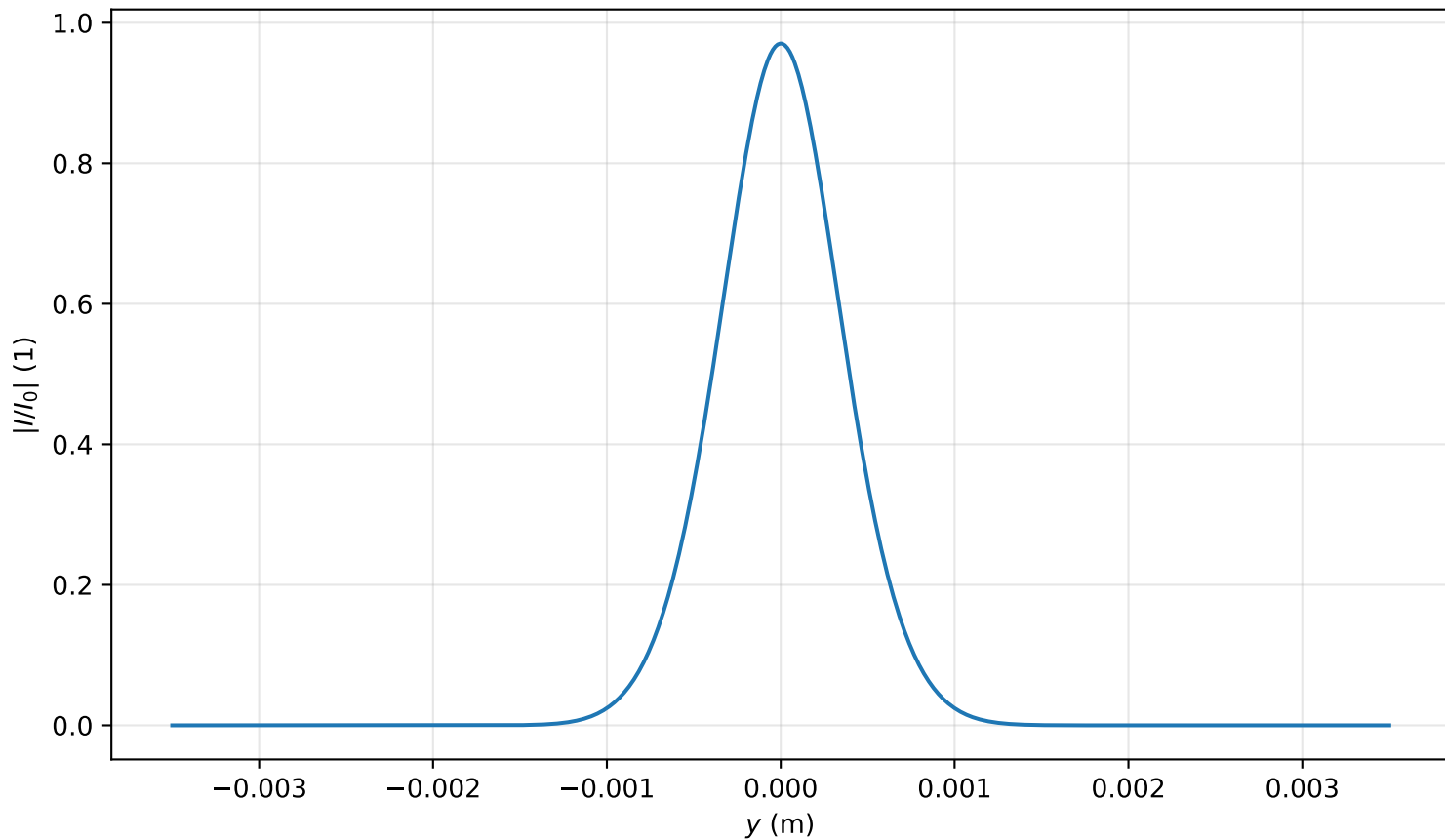
Intensity profile I(x=0, y, z=0.796)/I_0 , P_{in}=0.3P_{cr} , artificial time
